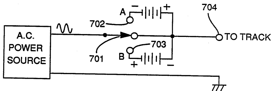
FIG. 7 \pm D.C. SIGNAL GENERATORS
