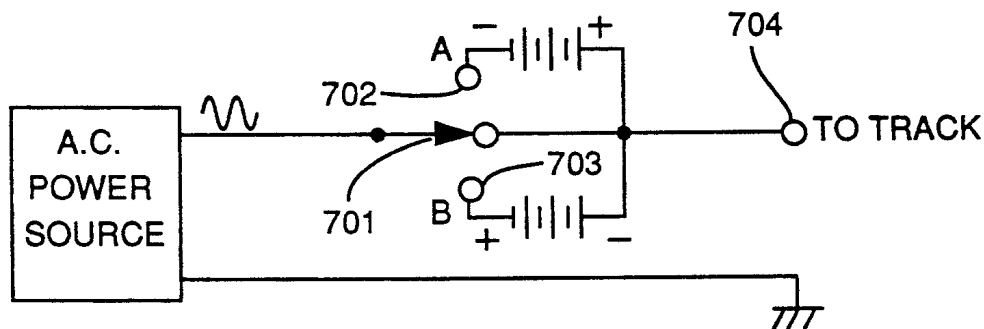
FIG. 7 \pm D.C. SIGNAL GENERATORS
