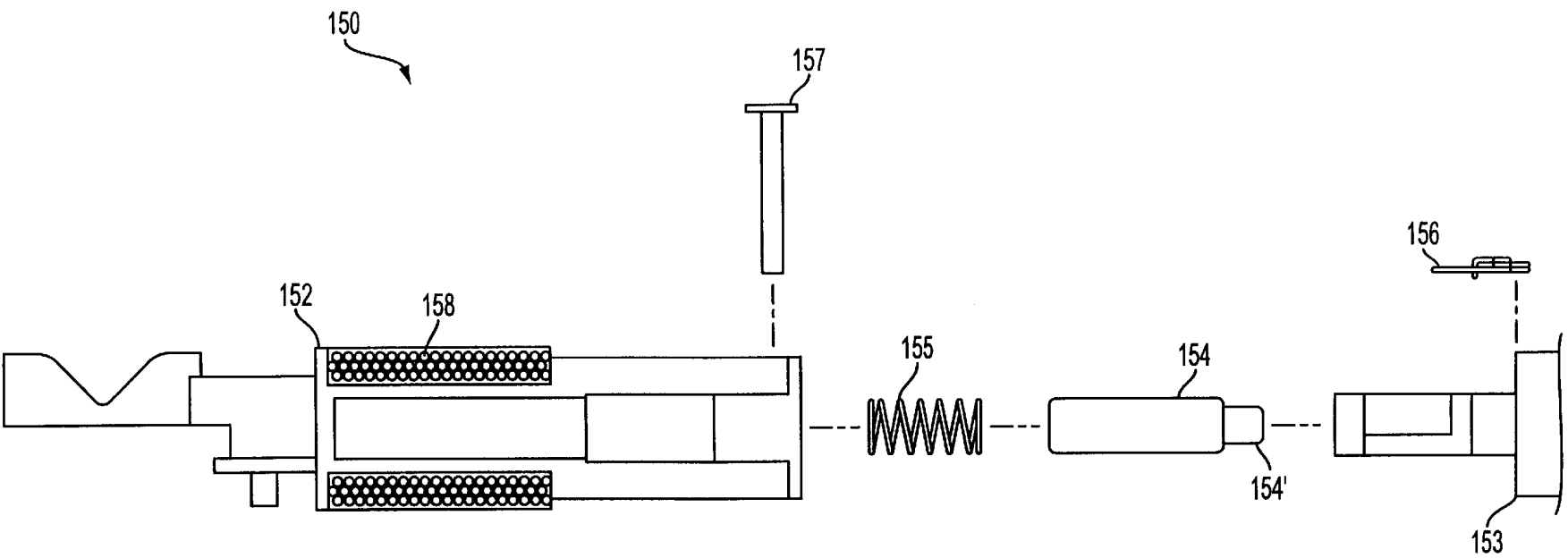
FIG. 12A (PRIOR ART)
