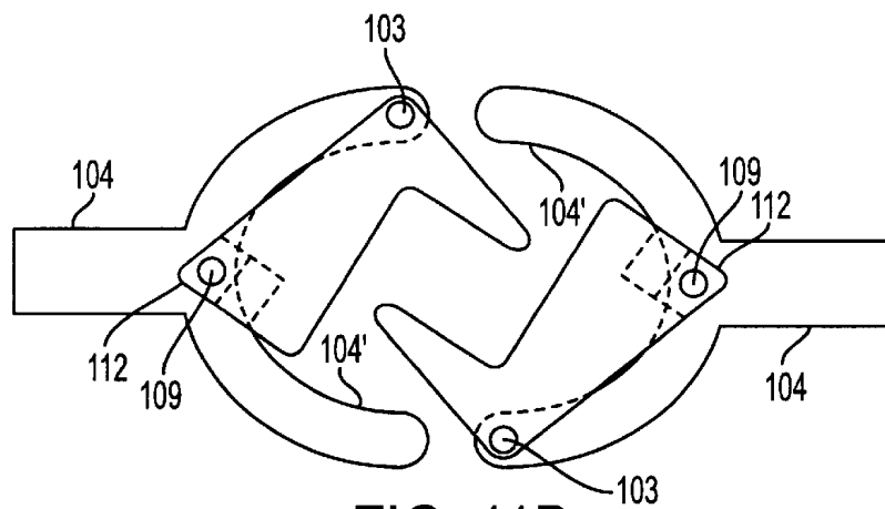
FIG. 11B (PRIOR ART)
