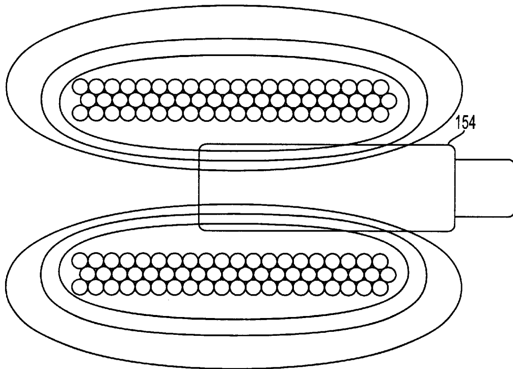
FIG. 13F (PRIOR ART)
